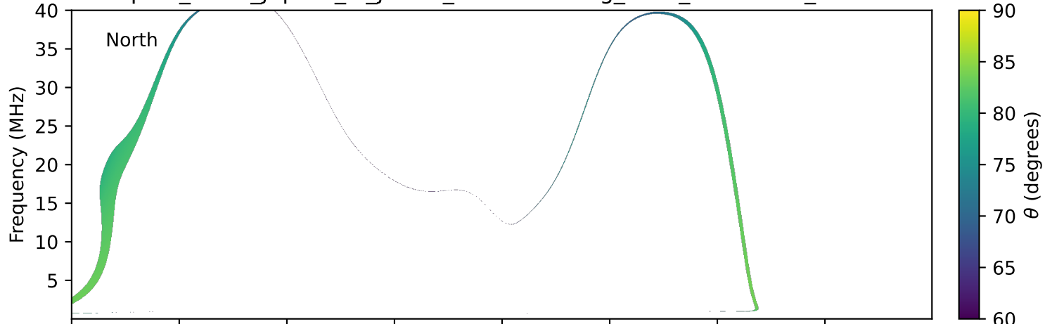
expres_earth_jupiter_io_jrm33_lossc-wid1deg_3kev_19951130_v11.cdf
