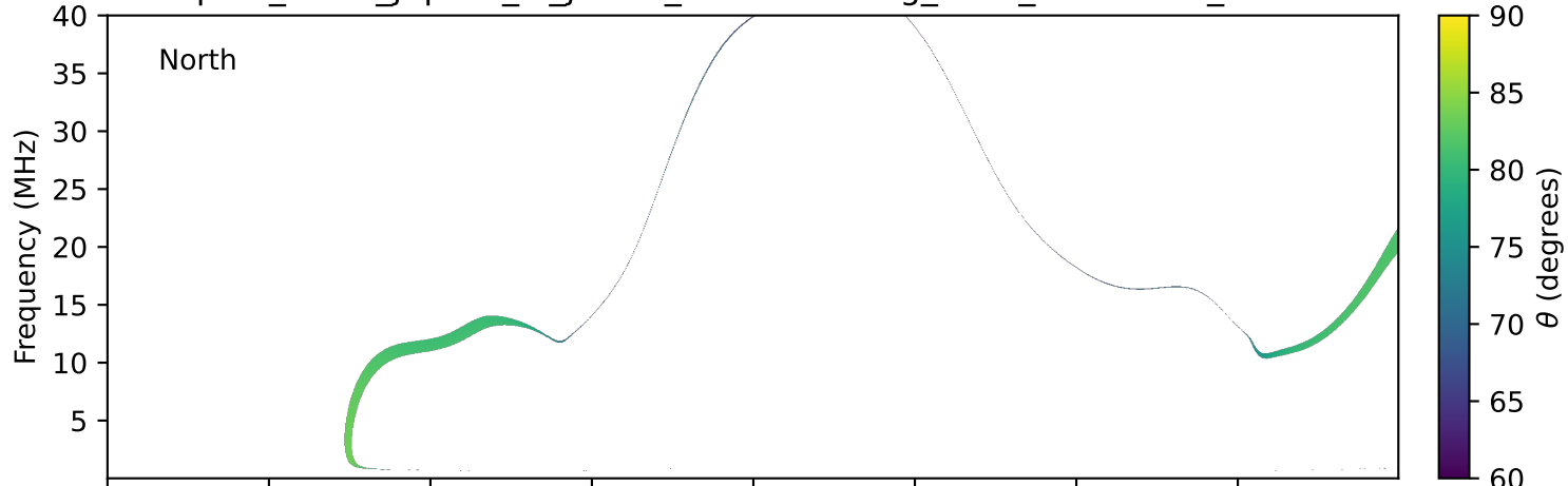
expres_earth_jupiter_io_jrm33_lossc-wid1deg_3kev_19951128_v11.cdf
