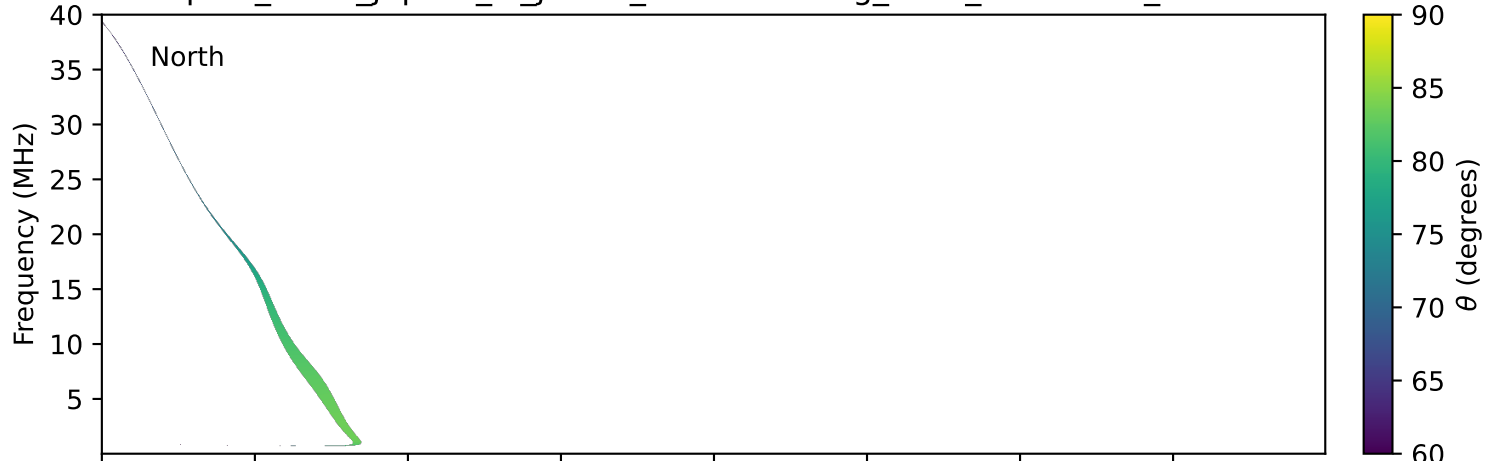
expres_earth_jupiter_io_jrm33_lossc-wid1deg_3kev_19951127_v11.cdf
