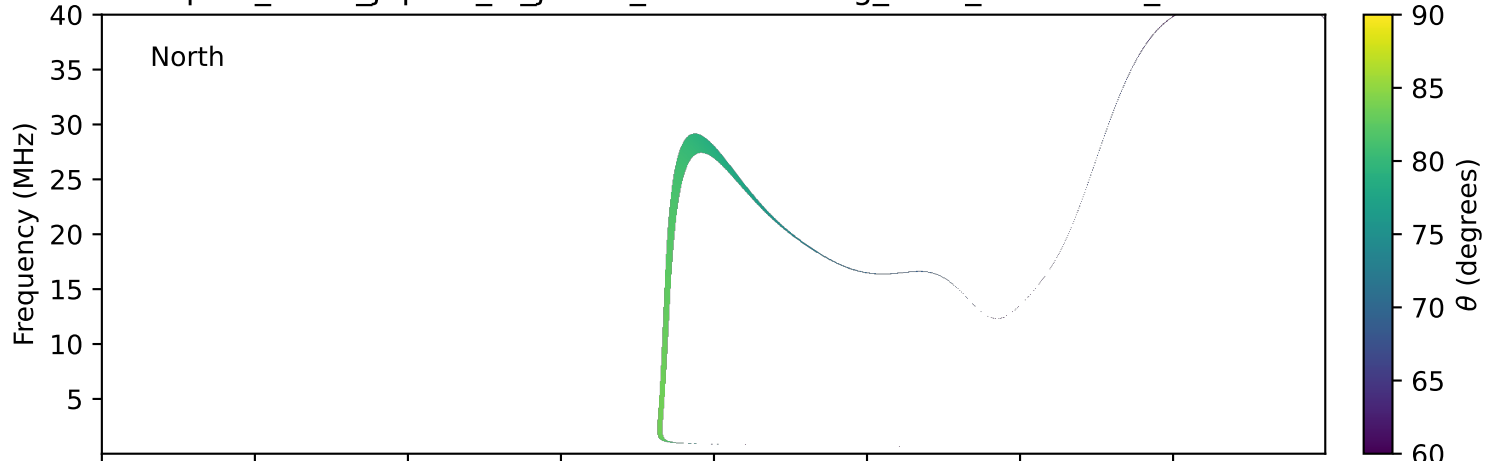
expres_earth_jupiter_io_jrm33_lossc-wid1deg_3kev_19951126_v11.cdf
