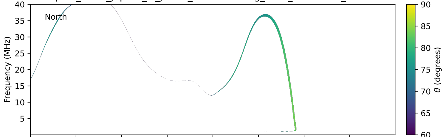
expres_earth_jupiter_io_jrm33_lossc-wid1deg_3kev_19951123_v11.cdf
