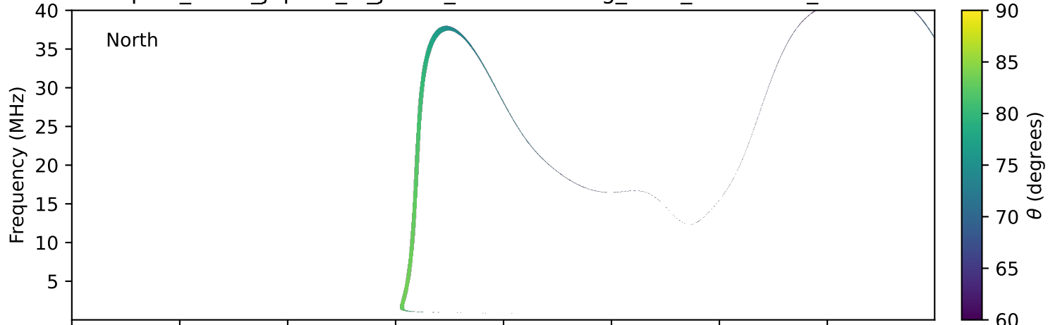
expres_earth_jupiter_io_jrm33_lossc-wid1deg_3kev_19951119_v11.cdf
