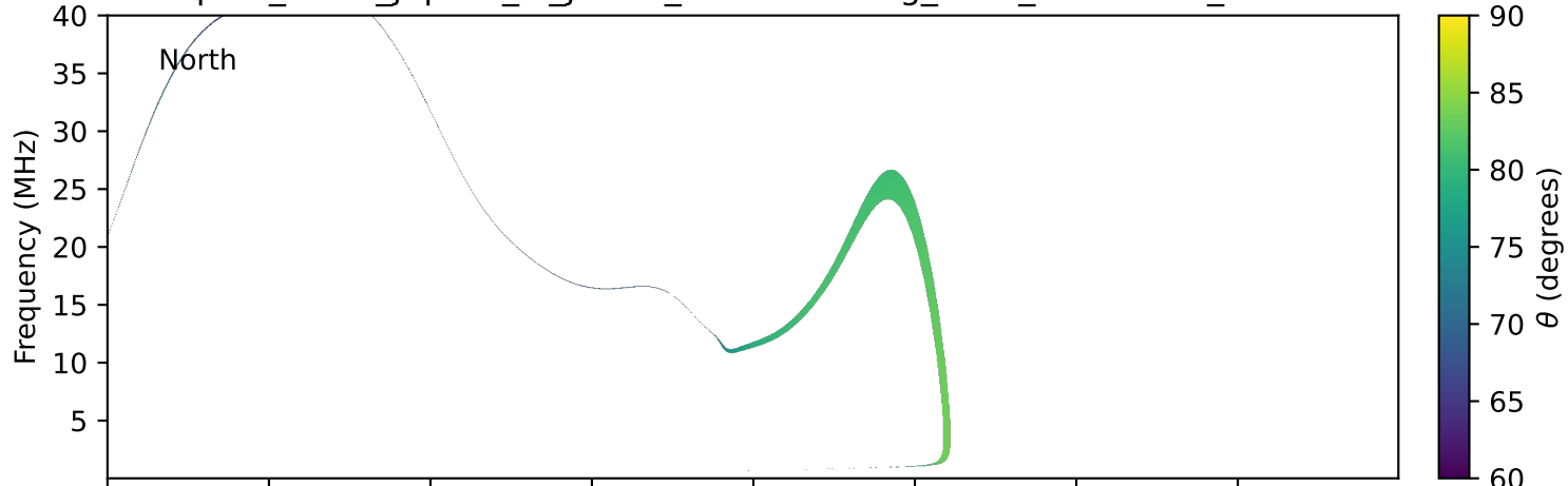
expres_earth_jupiter_io_jrm33_lossc-wid1deg_3kev_19951116_v11.cdf
