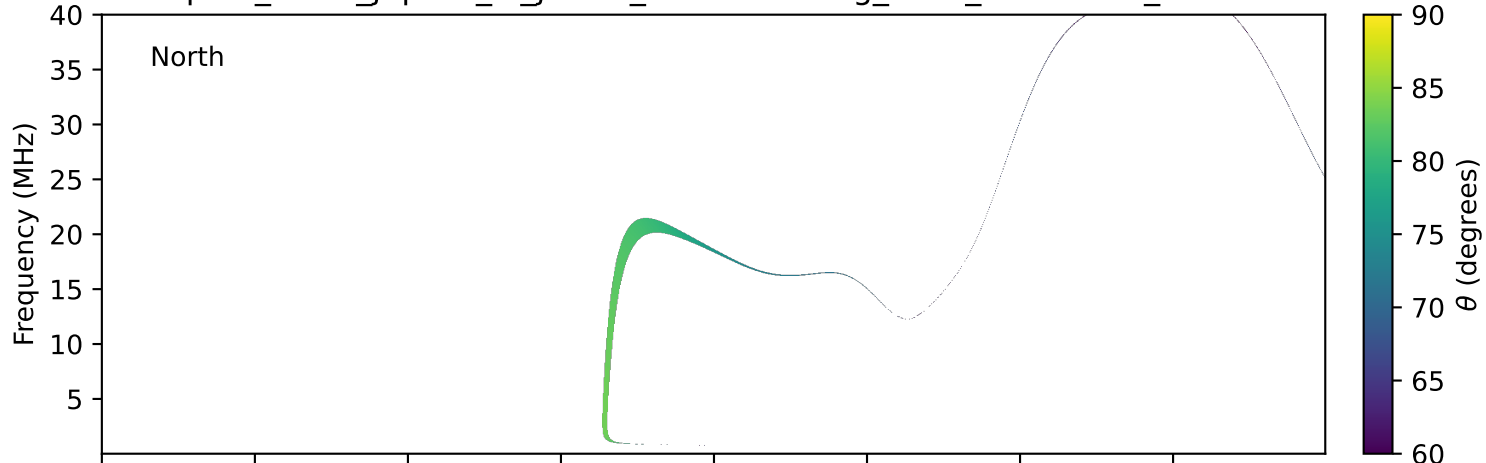
expres_earth_jupiter_io_jrm33_lossc-wid1deg_3kev_19951112_v11.cdf
