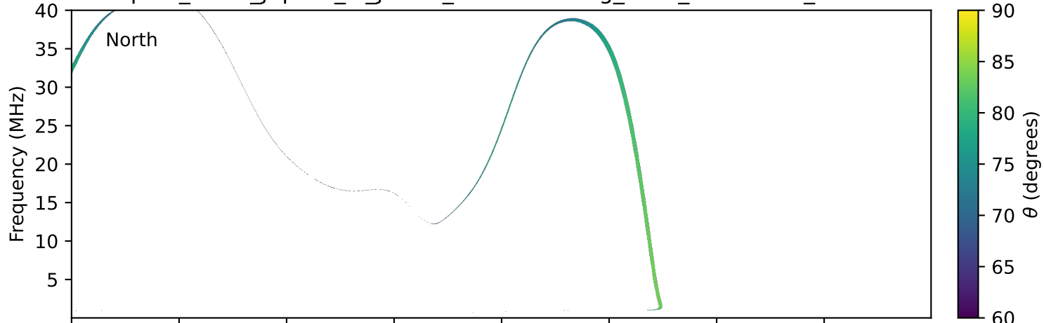
expres_earth_jupiter_io_jrm33_lossc-wid1deg_3kev_19951109_v11.cdf
