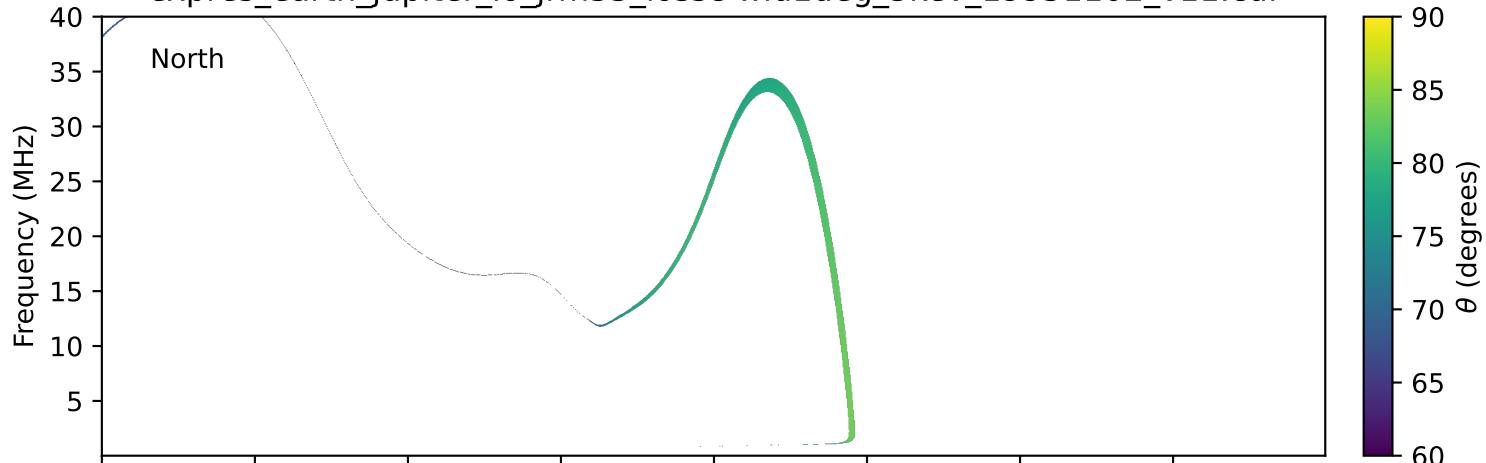
expres_earth_jupiter_io_jrm33_lossc-wid1deg_3kev_19951102_v11.cdf
