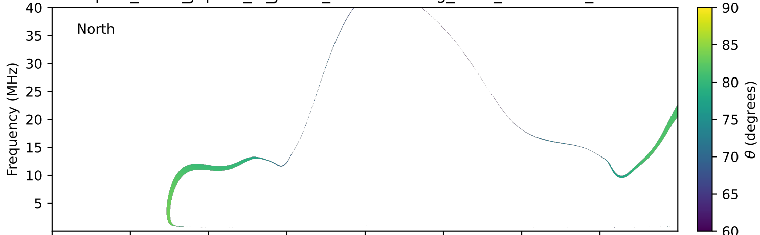
expres_earth_jupiter_io_jrm09_lossc-wid1deg_3kev_19951128_v11.cdf
