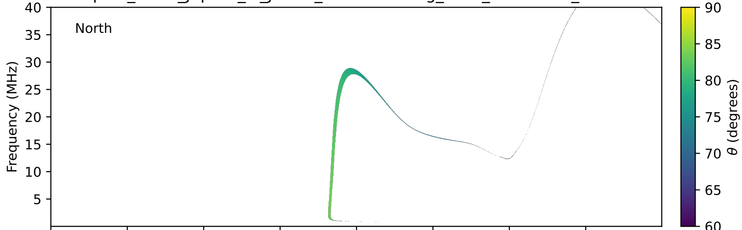
expres_earth_jupiter_io_jrm09_lossc-wid1deg_3kev_19951126_v11.cdf
