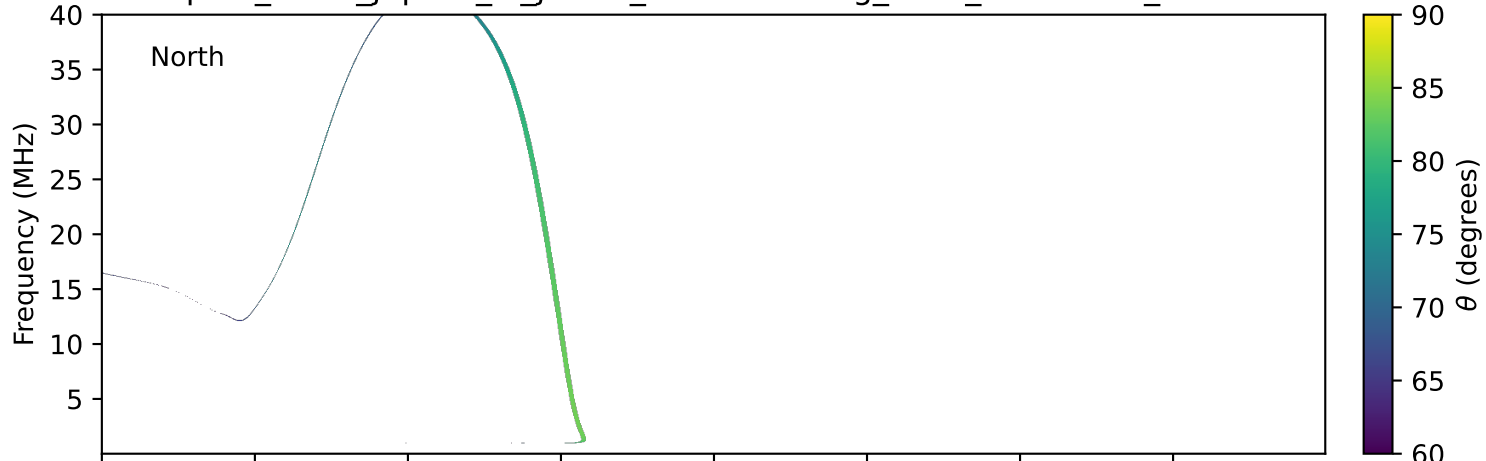
expres_earth_jupiter_io_jrm09_lossc-wid1deg_3kev_19951118_v11.cdf
