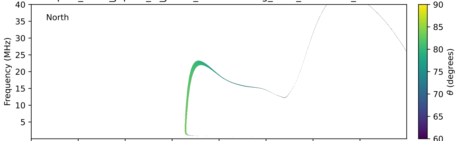
expres_earth_jupiter_io_jrm09_lossc-wid1deg_3kev_19951112_v11.cdf
