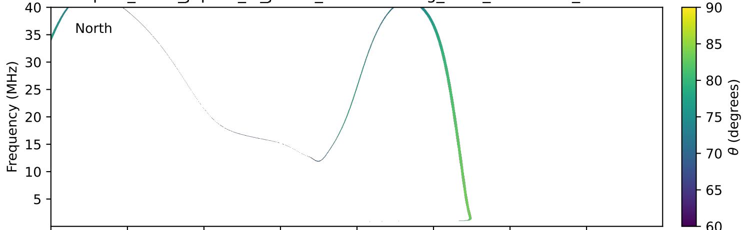
expres_earth_jupiter_io_jrm09_lossc-wid1deg_3kev_19951109_v11.cdf
