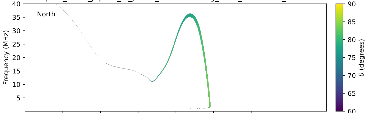
expres_earth_jupiter_io_jrm09_lossc-wid1deg_3kev_19951102_v11.cdf
