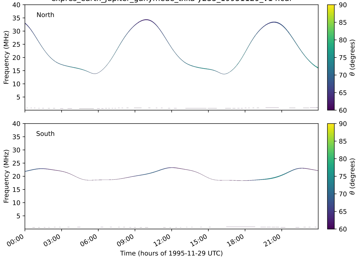
expres_earth_jupiter_ganymede_txka-y235_19951129_v14.cdf
