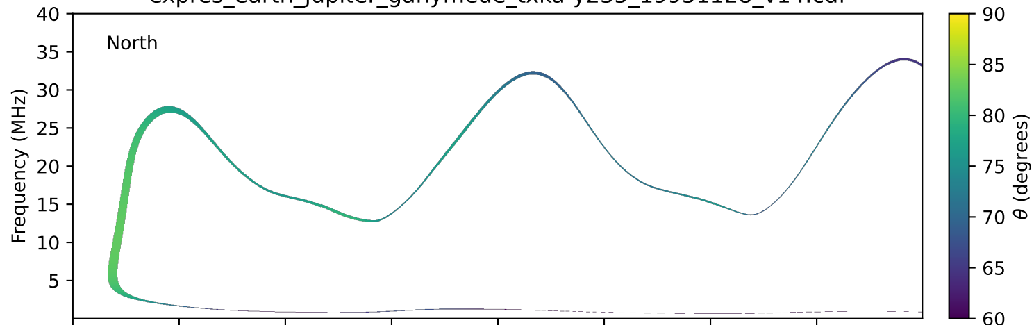
expres_earth_jupiter_ganymede_txka-y235_19951128_v14.cdf
