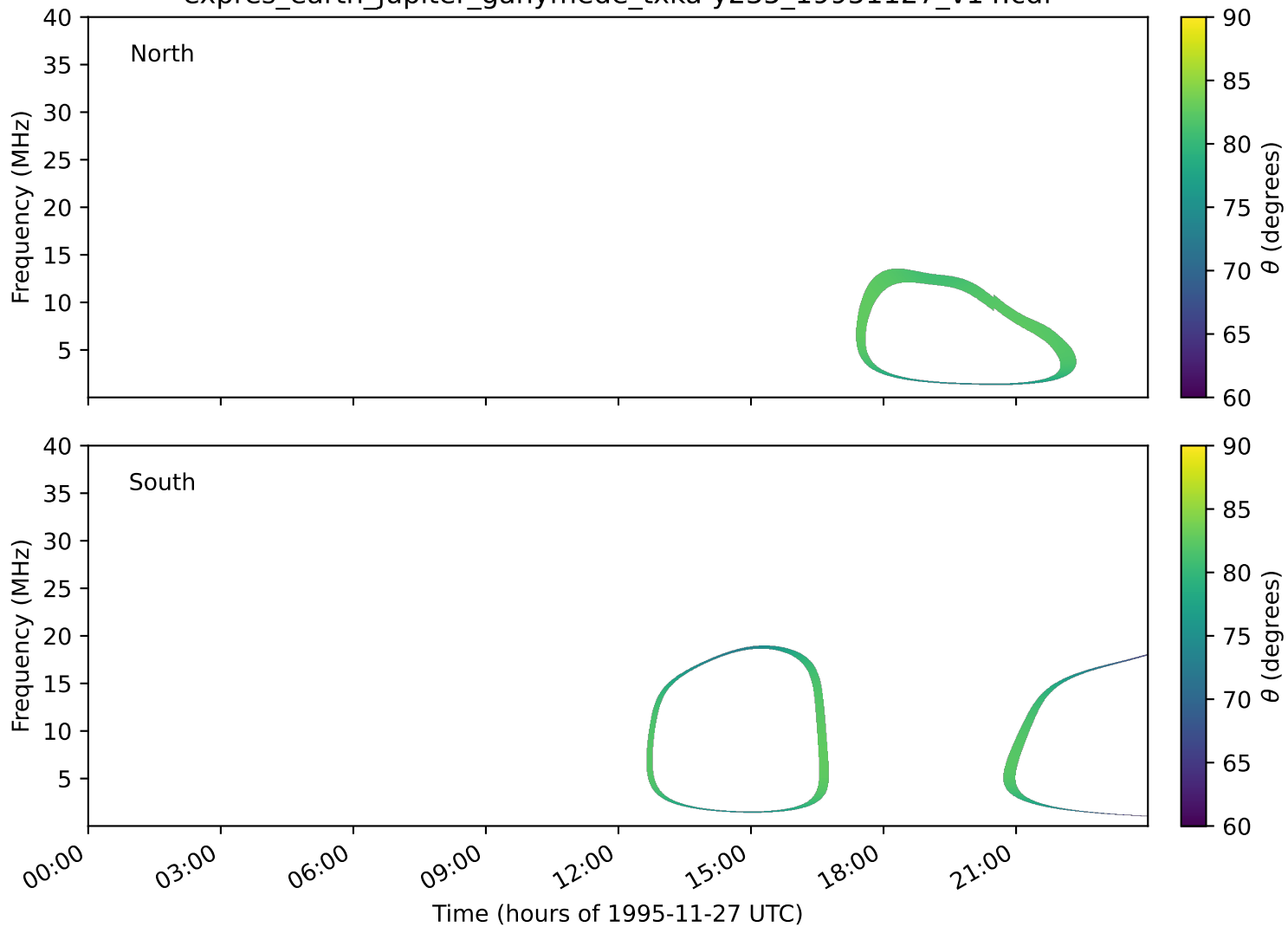
expres_earth_jupiter_ganymede_txka-y235_19951127_v14.cdf
