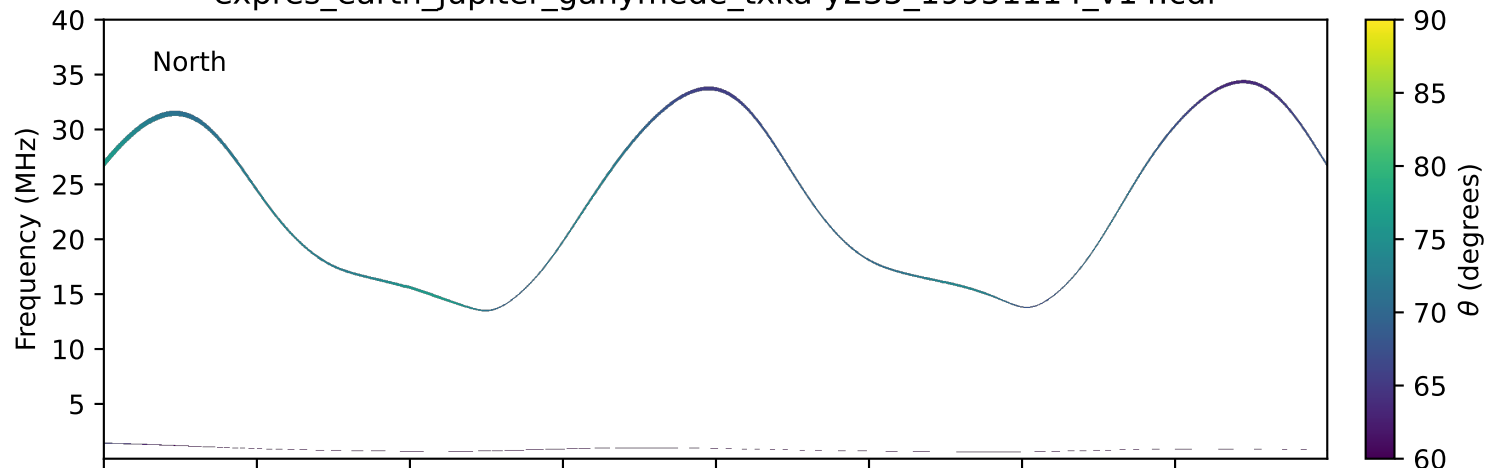
expres_earth_jupiter_ganymede_txka-y235_19951114_v14.cdf
