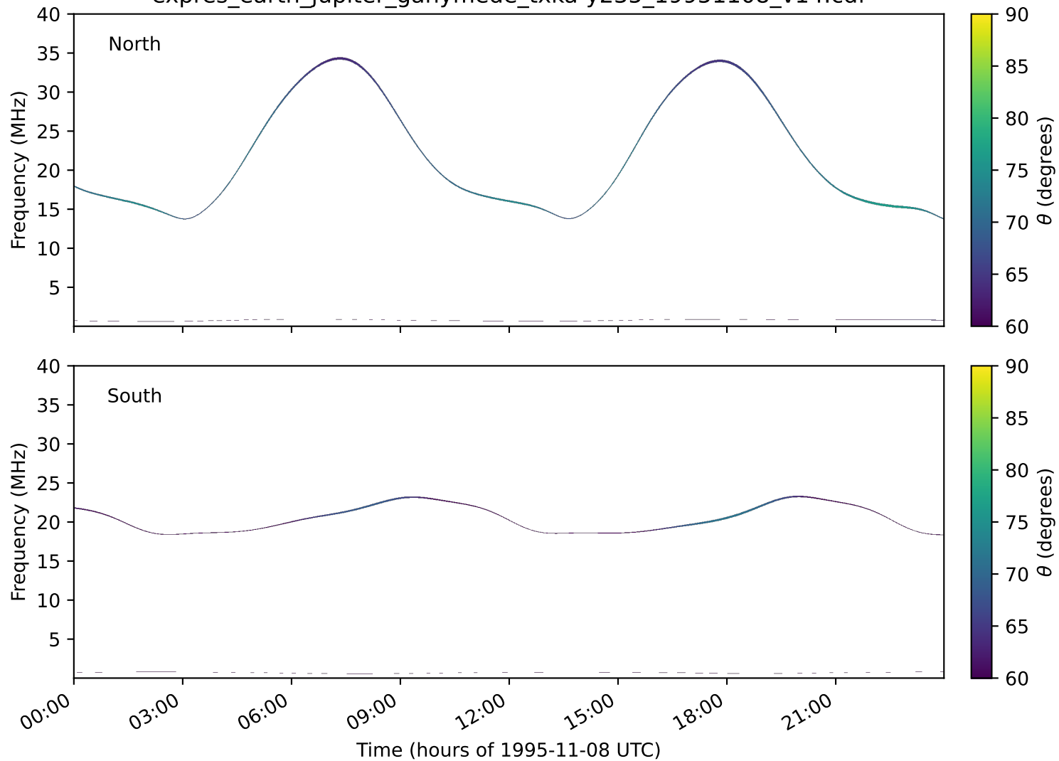
expres_earth_jupiter_ganymede_txka-y235_19951108_v14.cdf
