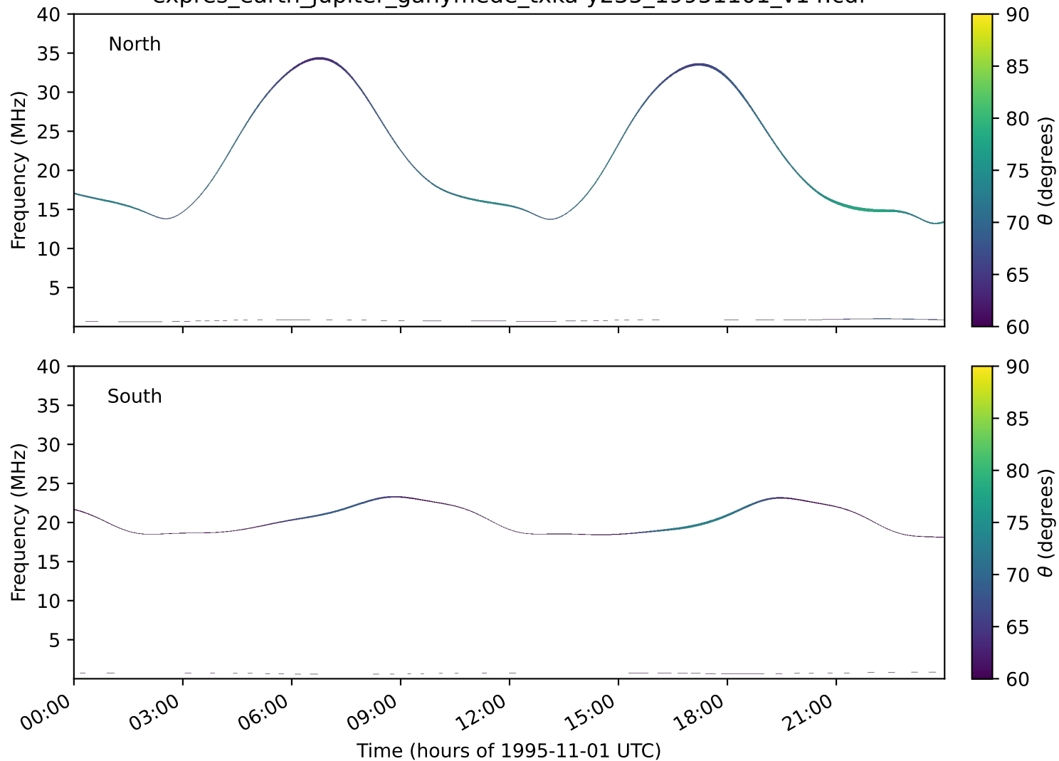
expres_earth_jupiter_ganymede_txka-y235_19951101_v14.cdf
