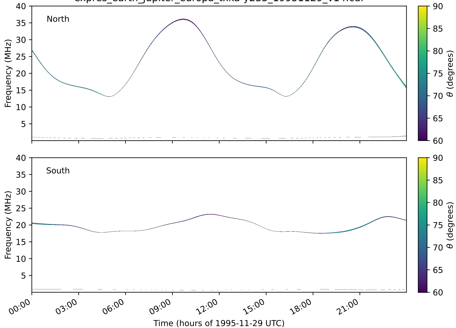
expres_earth_jupiter_europa_txka-y235_19951129_v14.cdf
