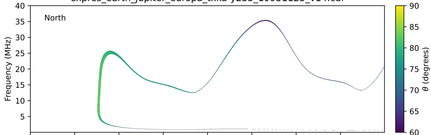
expres_earth_jupiter_europa_txka-y235_19951125_v14.cdf
