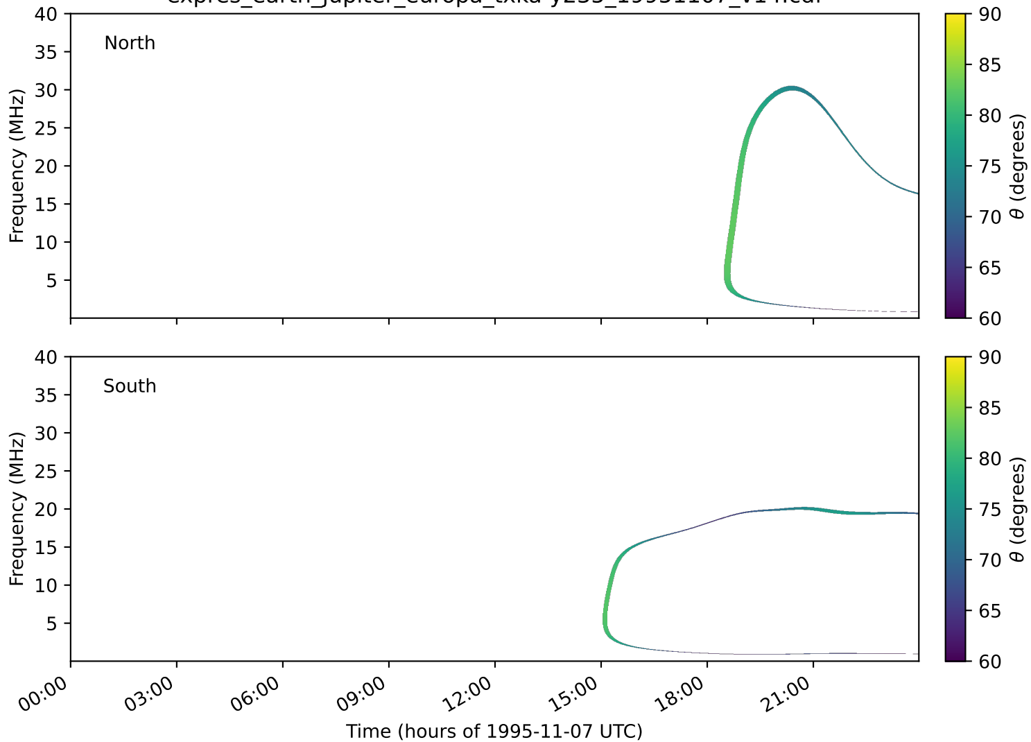
expres_earth_jupiter_europa_txka-y235_19951107_v14.cdf
