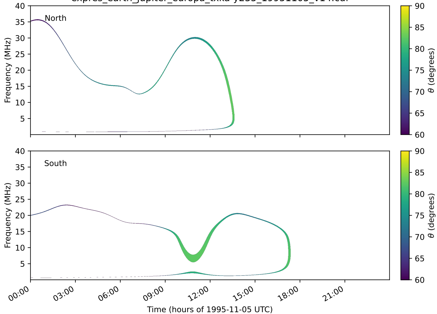
expres_earth_jupiter_europa_txka-y235_19951105_v14.cdf
