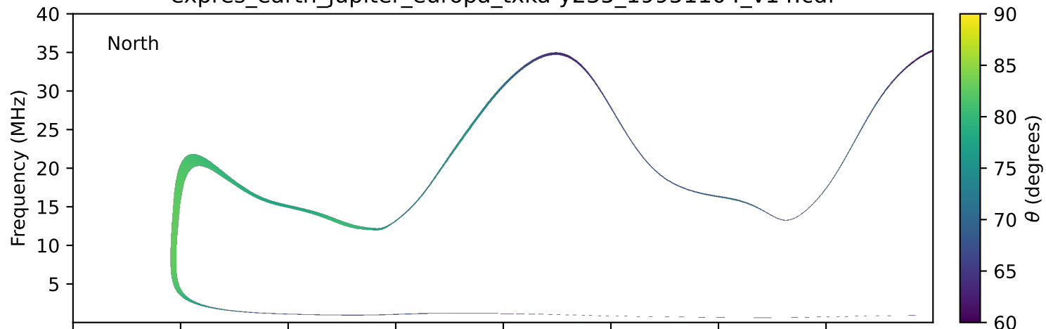
expres_earth_jupiter_europa_txka-y235_19951104_v14.cdf
