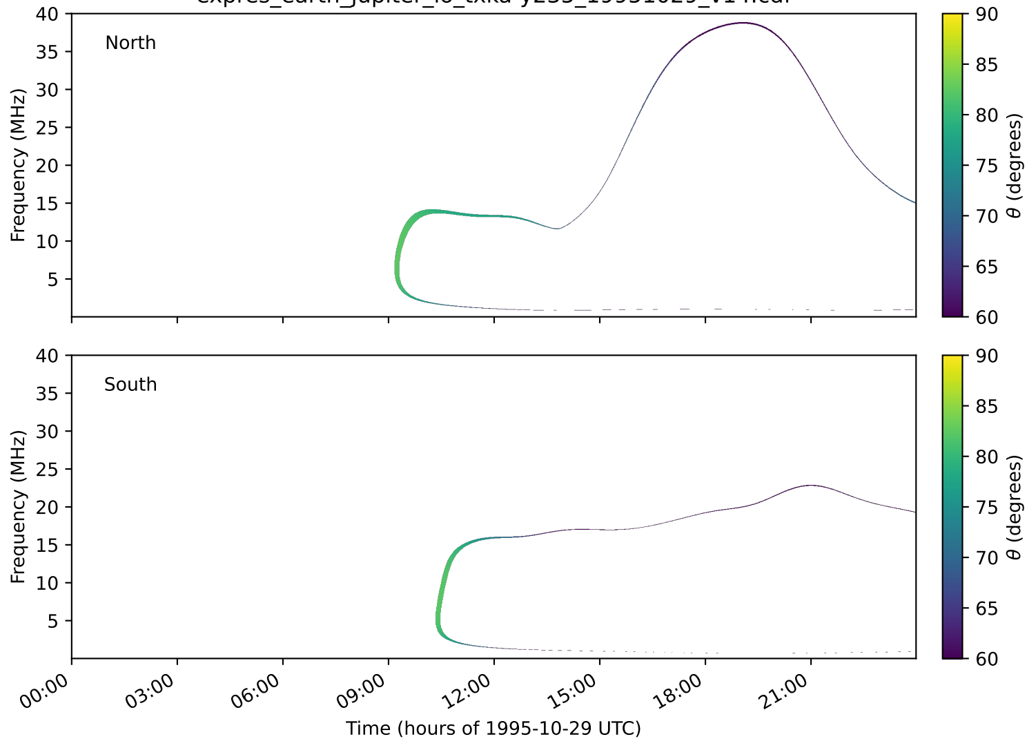
expres_earth_jupiter_io_txka-y235_19951029_v14.cdf
