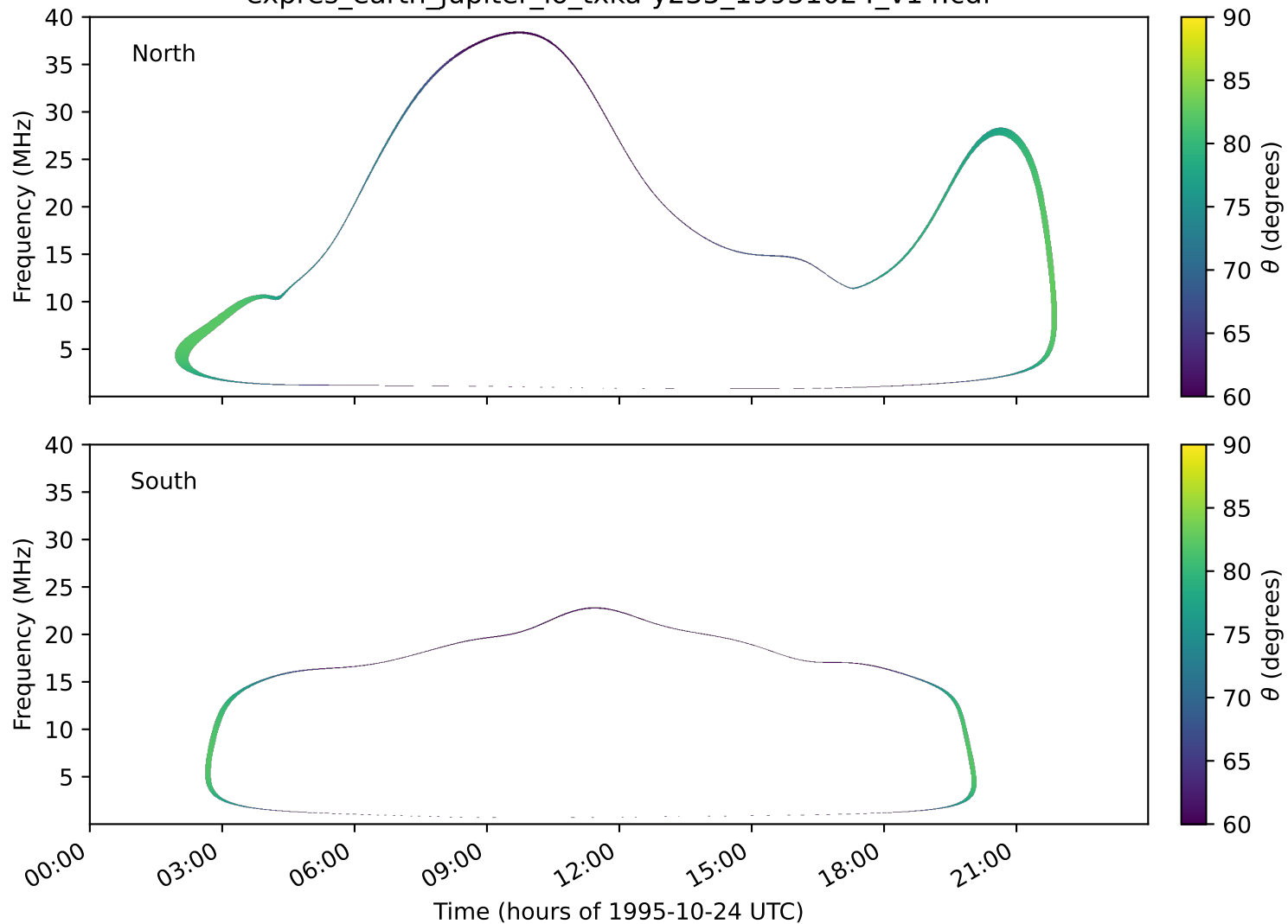
expres_earth_jupiter_io_txka-y235_19951024_v14.cdf
