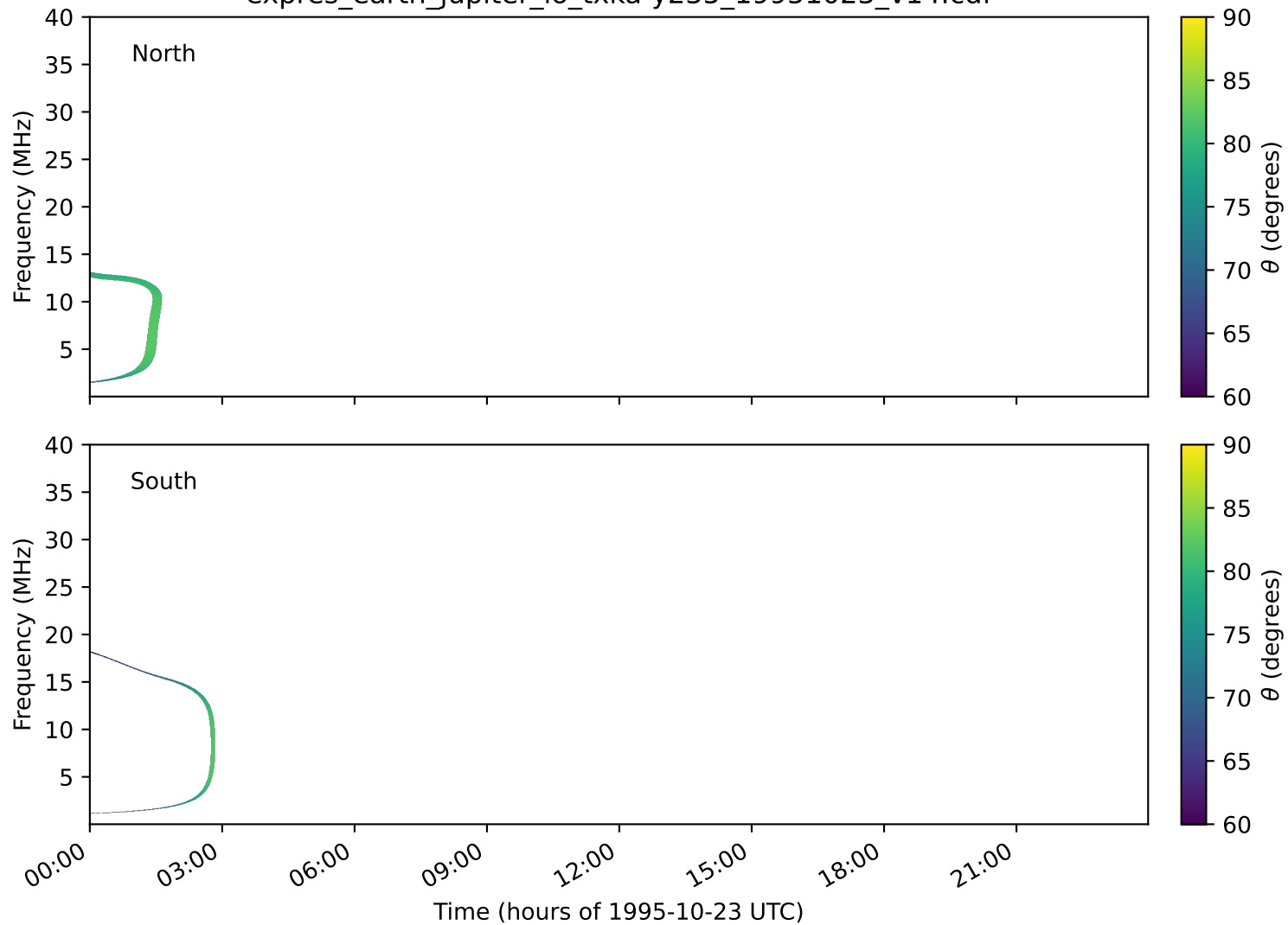
expres_earth_jupiter_io_txka-y235_19951023_v14.cdf
