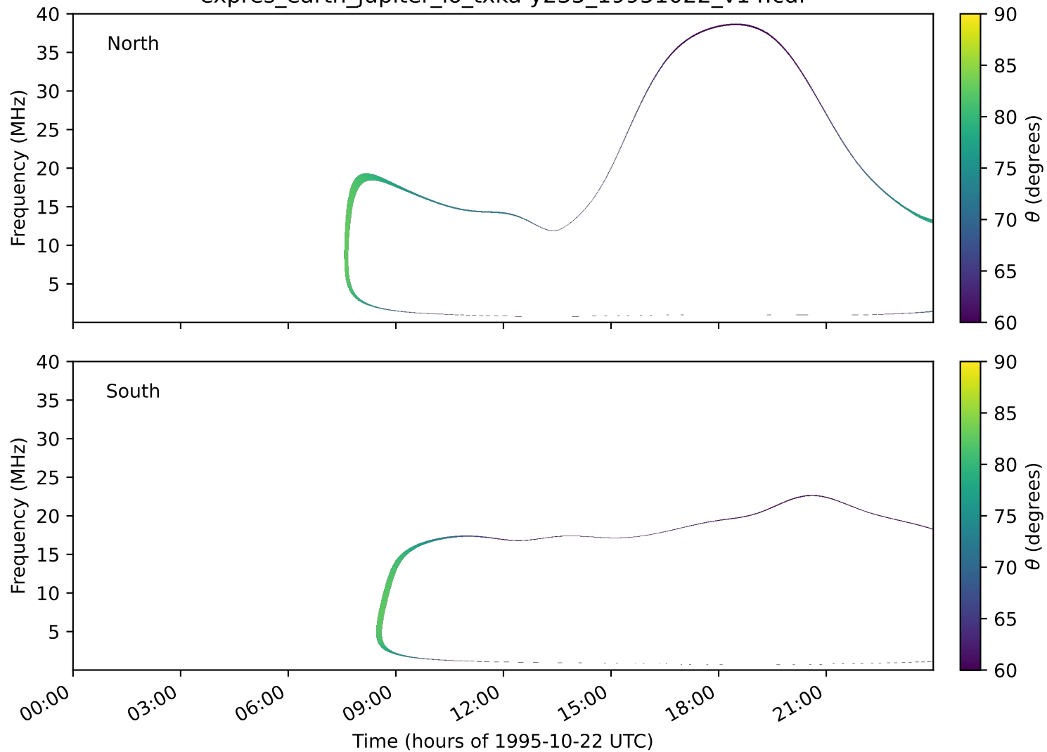
expres_earth_jupiter_io_txka-y235_19951022_v14.cdf
