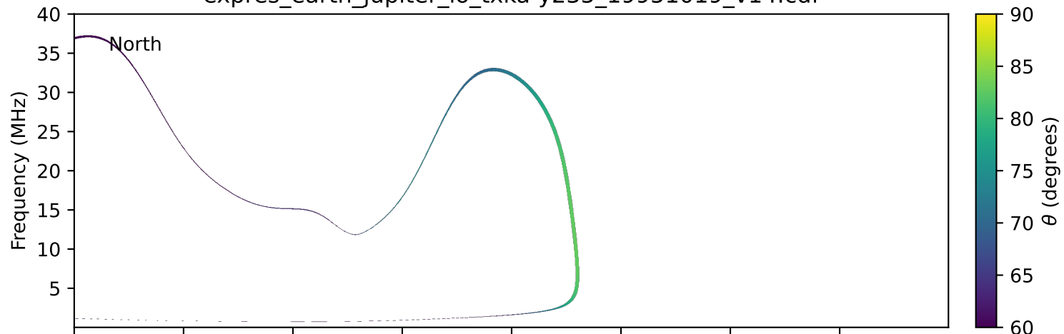
expres_earth_jupiter_io_txka-y235_19951019_v14.cdf
