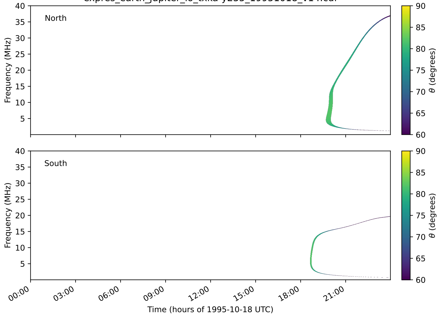
expres_earth_jupiter_io_txka-y235_19951018_v14.cdf
