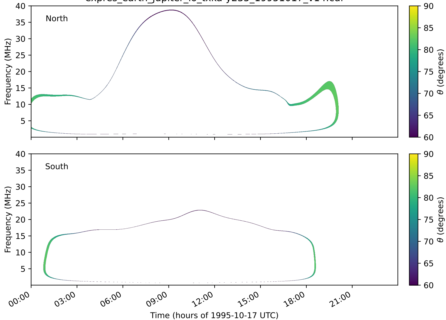
expres_earth_jupiter_io_txka-y235_19951017_v14.cdf
