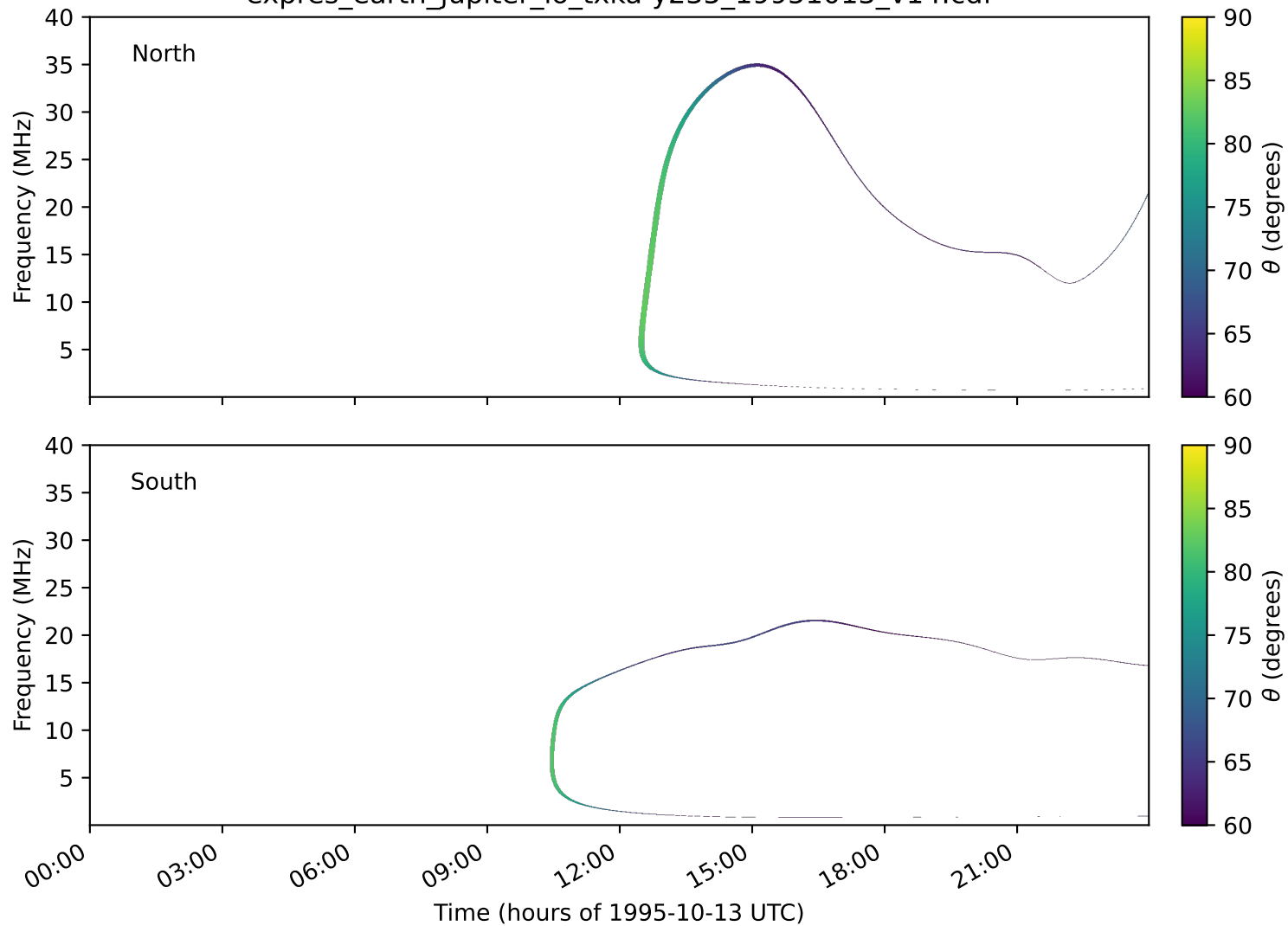
expres_earth_jupiter_io_txka-y235_19951013_v14.cdf
