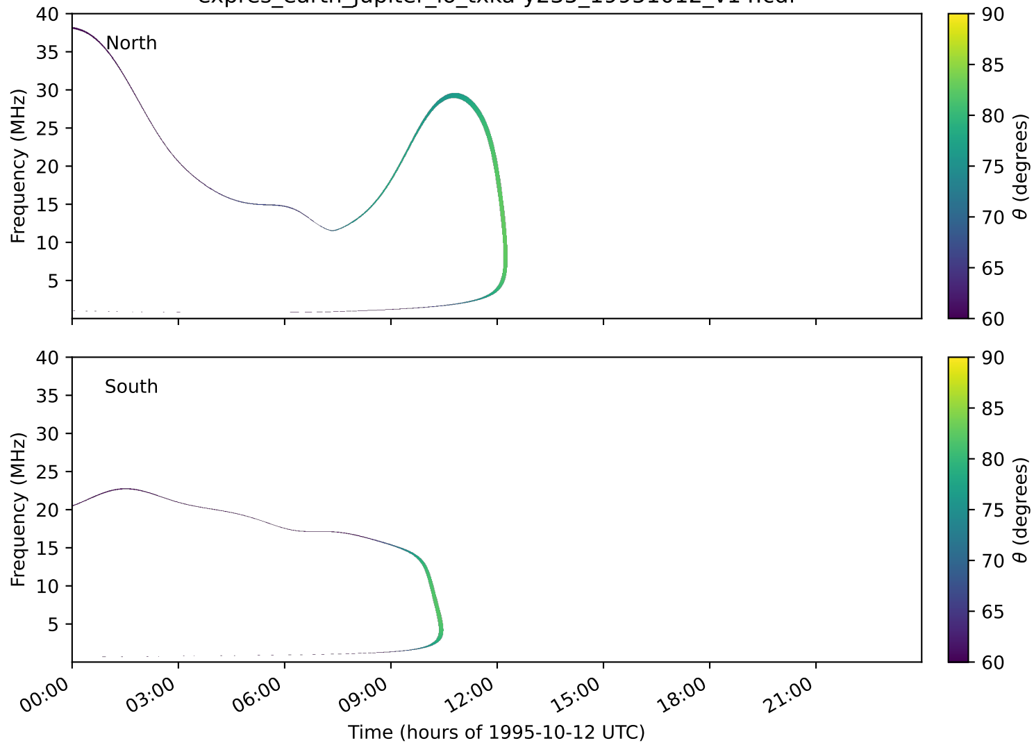
expres_earth_jupiter_io_txka-y235_19951012_v14.cdf
