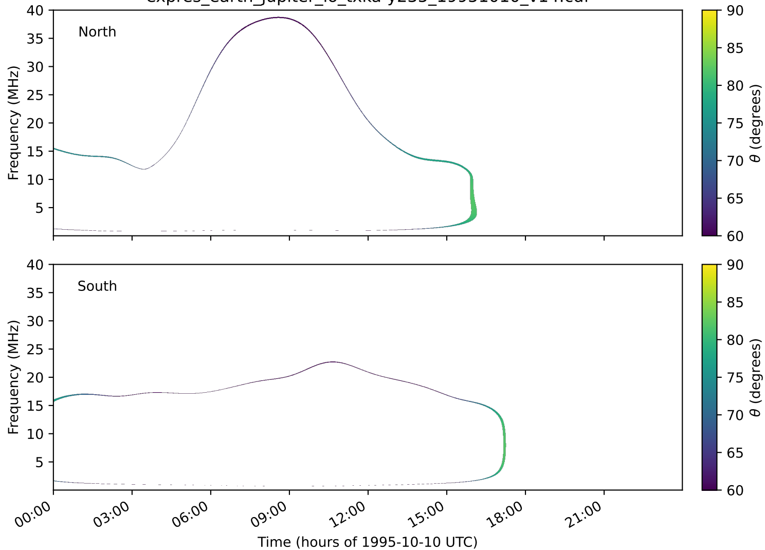
expres_earth_jupiter_io_txka-y235_19951010_v14.cdf
