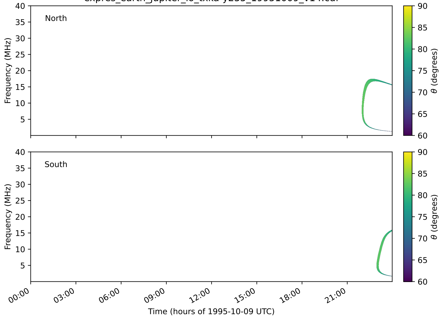
expres_earth_jupiter_io_txka-y235_19951009_v14.cdf
