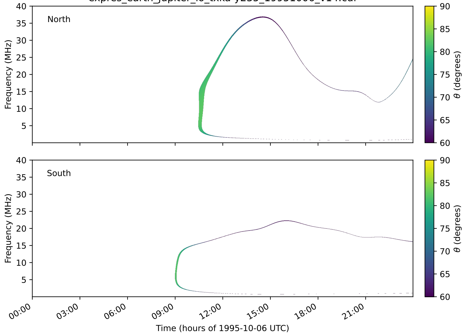
expres_earth_jupiter_io_txka-y235_19951006_v14.cdf
