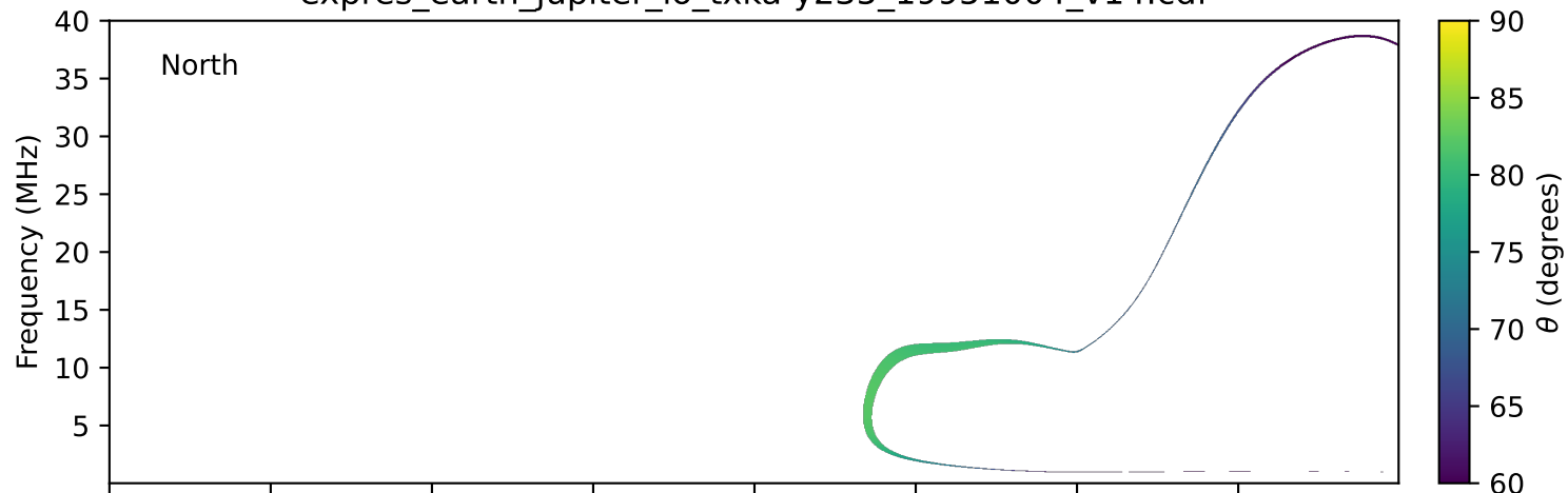
expres_earth_jupiter_io_txka-y235_19951004_v14.cdf
