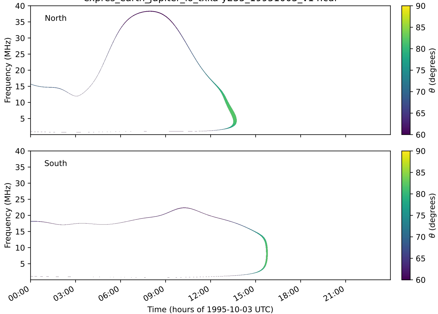
expres_earth_jupiter_io_txka-y235_19951003_v14.cdf
