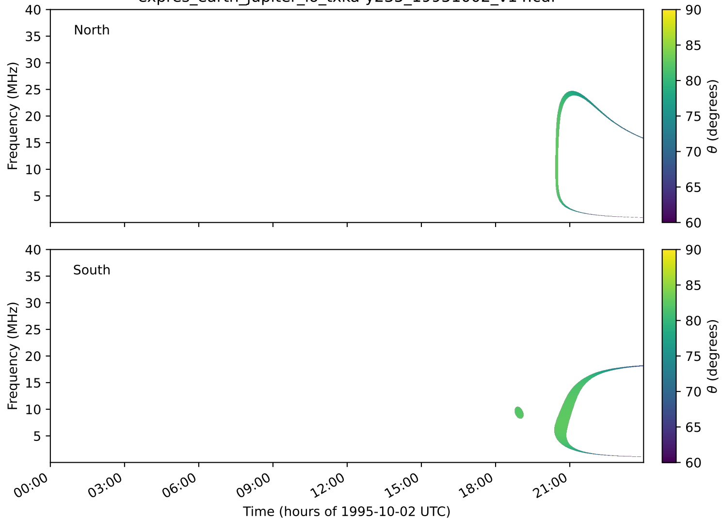
expres_earth_jupiter_io_txka-y235_19951002_v14.cdf
