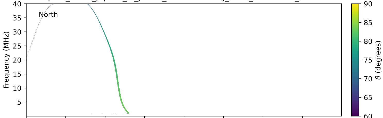
expres_earth_jupiter_io_jrm33_lossc-wid1deg_3kev_19951021_v11.cdf
