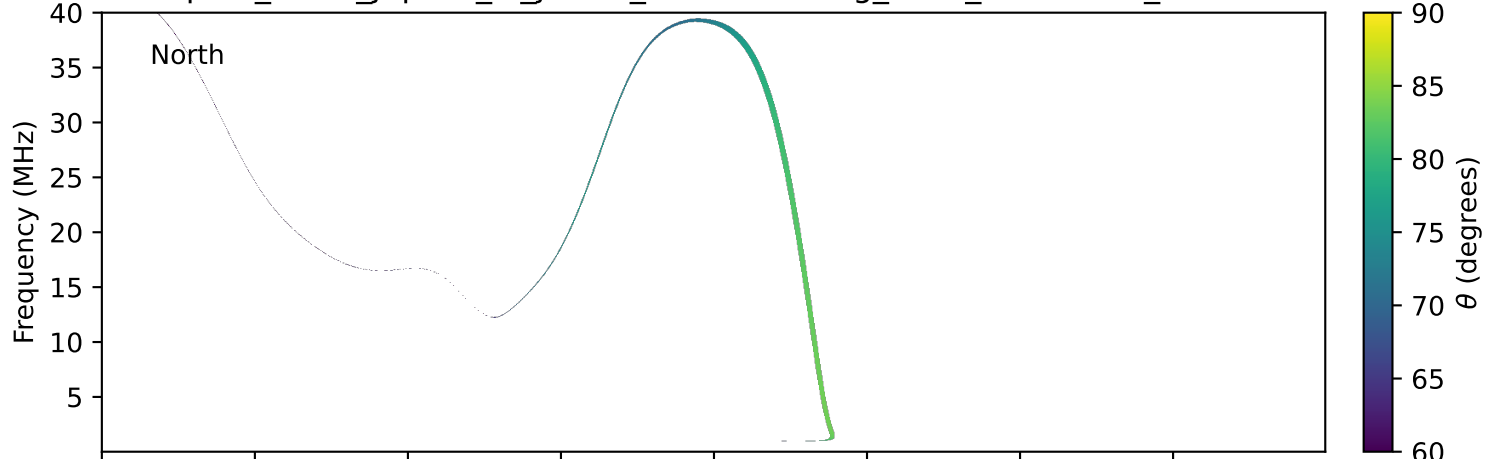
expres_earth_jupiter_io_jrm33_lossc-wid1deg_3kev_19951019_v11.cdf
