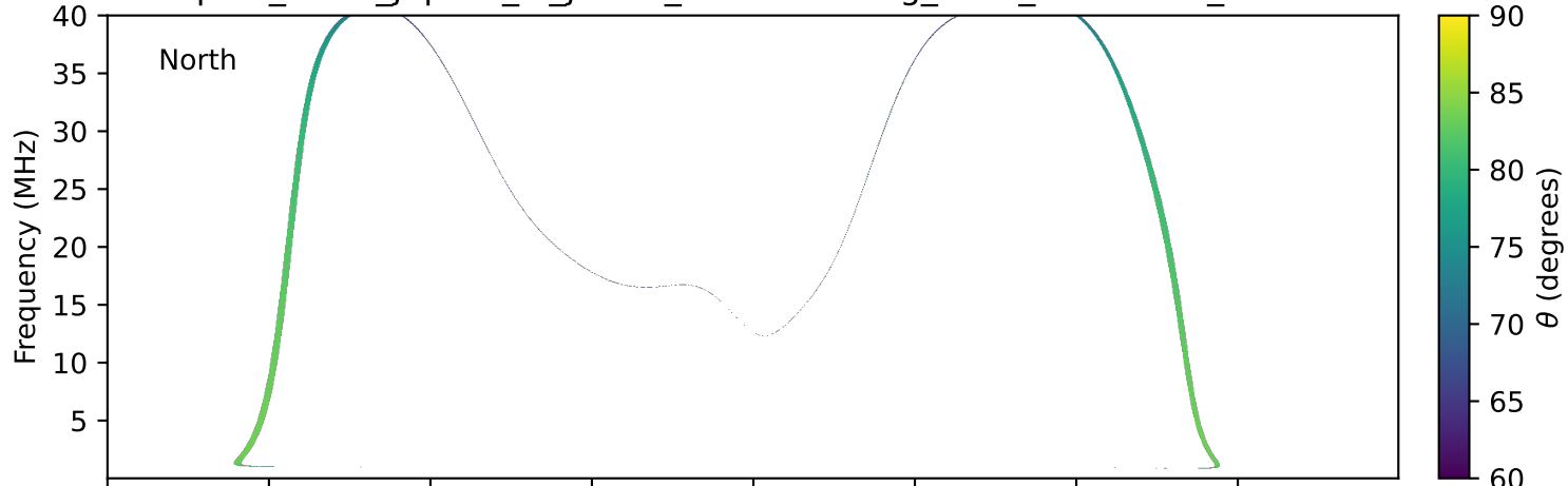
expres_earth_jupiter_io_jrm33_lossc-wid1deg_3kev_19951001_v11.cdf
