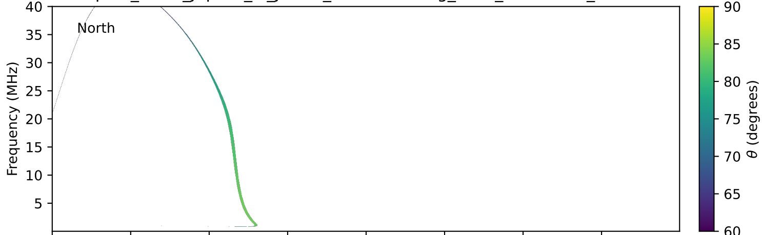
expres_earth_jupiter_io_jrm09_lossc-wid1deg_3kev_19951021_v11.cdf
