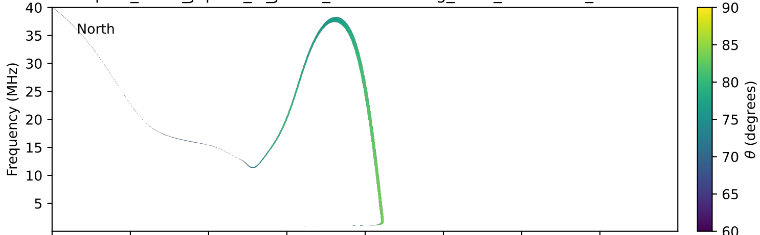
expres_earth_jupiter_io_jrm09_lossc-wid1deg_3kev_19951012_v11.cdf
