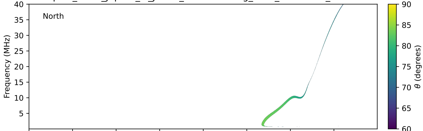
expres_earth_jupiter_io_jrm09_lossc-wid1deg_3kev_19951011_v11.cdf
