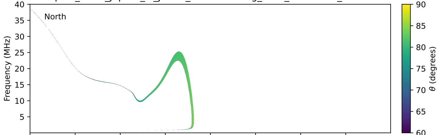
expres_earth_jupiter_io_jrm09_lossc-wid1deg_3kev_19951005_v11.cdf
