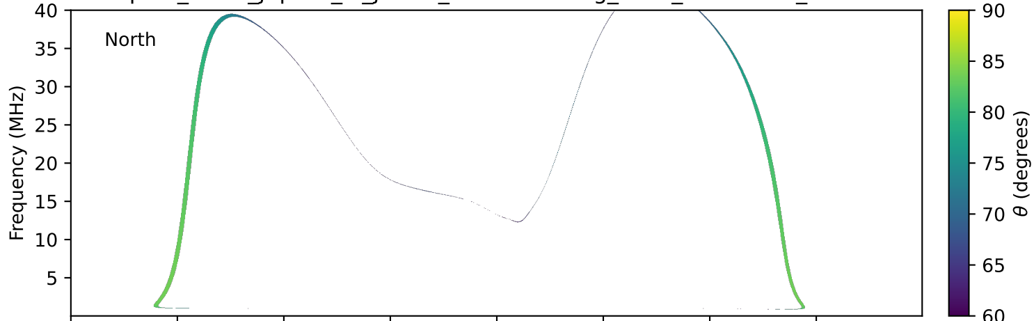
expres_earth_jupiter_io_jrm09_lossc-wid1deg_3kev_19951001_v11.cdf
